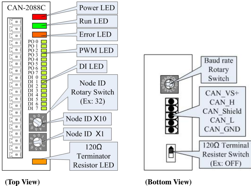
Figure 2-1 CAN-2088C layout of LED, connect, and switch
