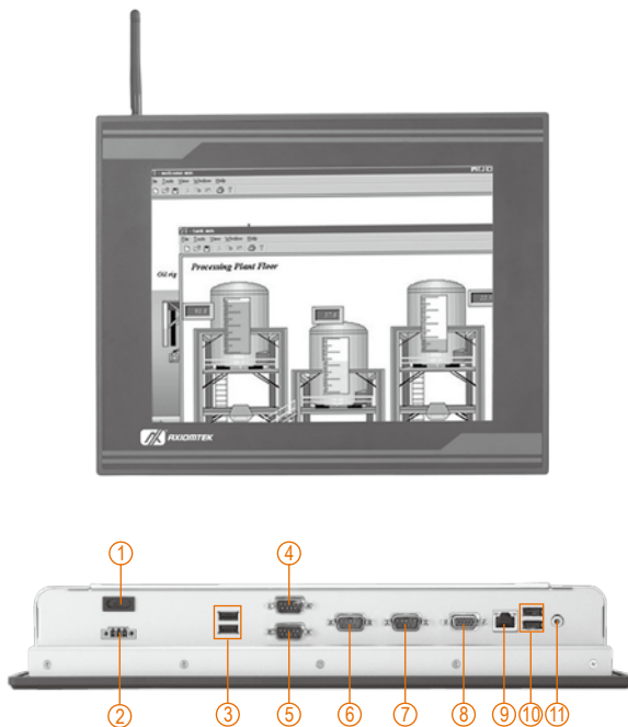
I/O of GOT-3156TL-830
