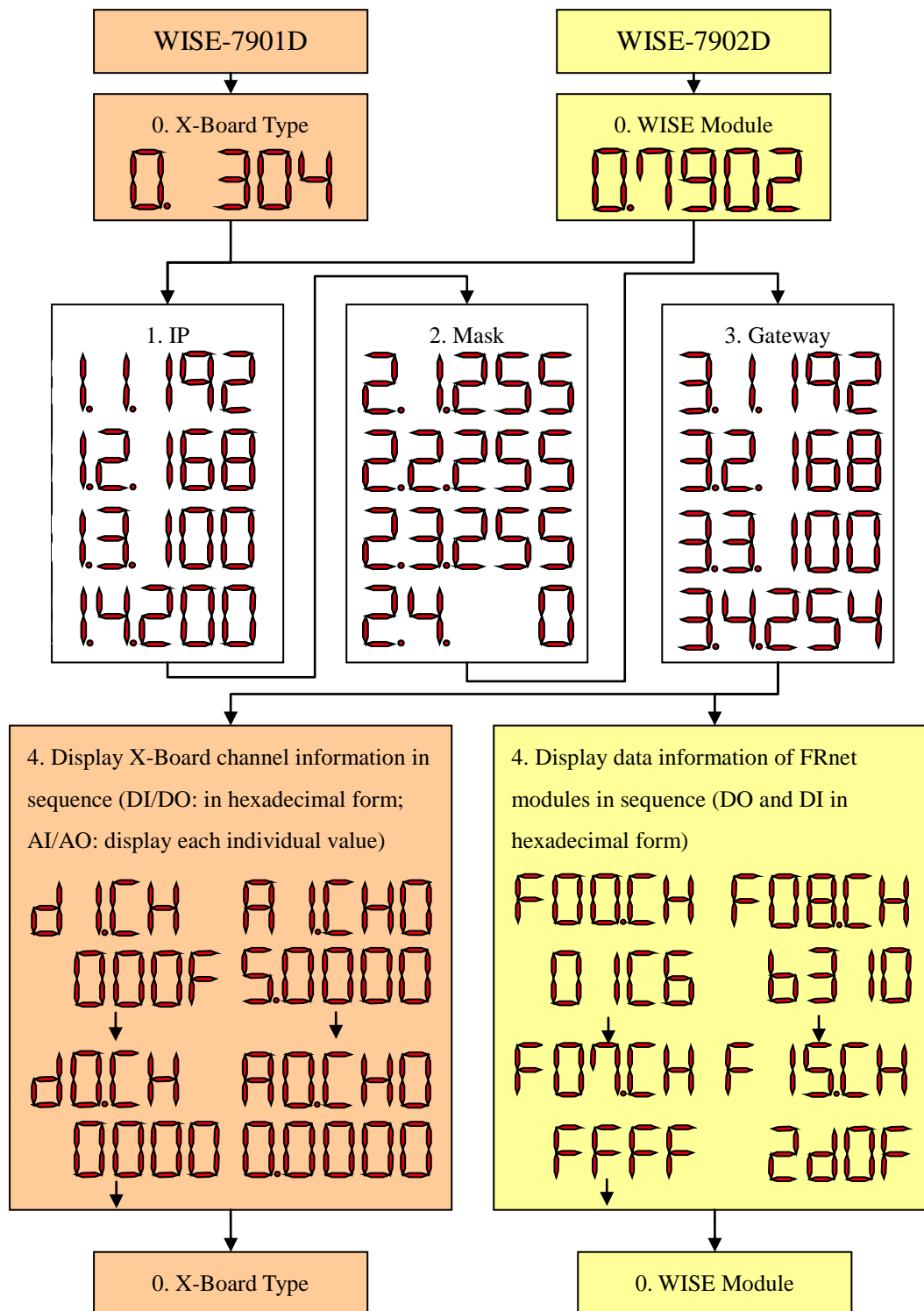
Figure 10-1 : The LED display shows network information and channel values
