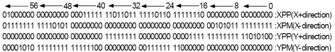
Fig. A-26 Bit pattern data for X-Y profile
