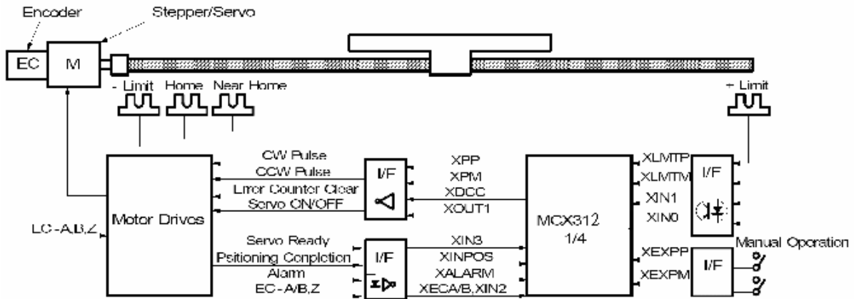
Fig. A-29 X-axis hardware signal disposition
