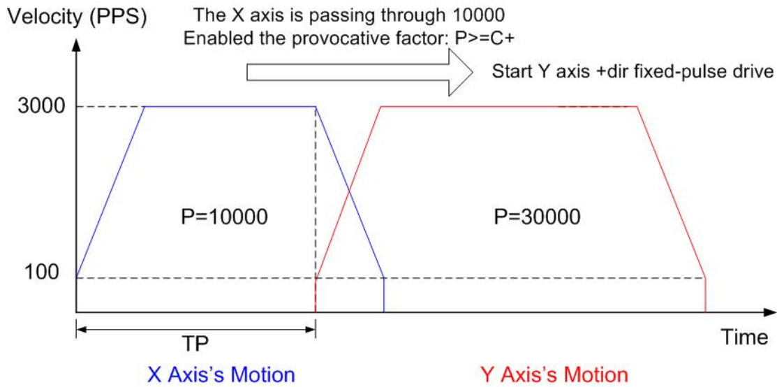
Fig. A-42 Synchronous action example 1
