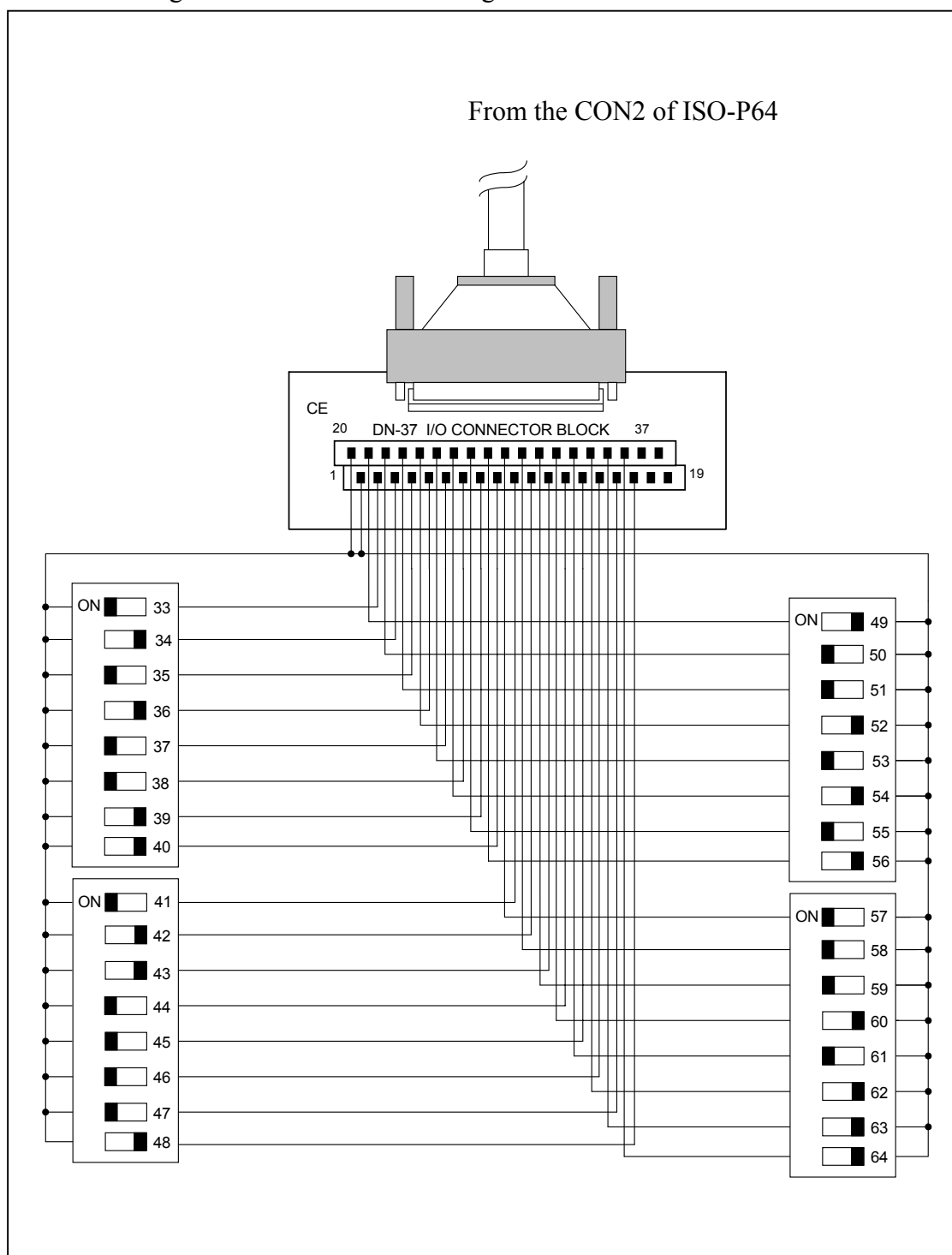
Figure 3-8. The circuit diagram of external device 2 for the digital inputs of ISO-P64
