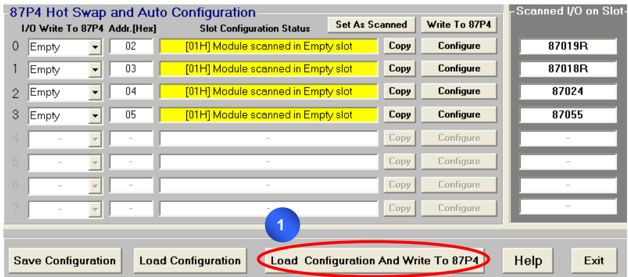
Fig. 19 : Load & Write the configuration file
