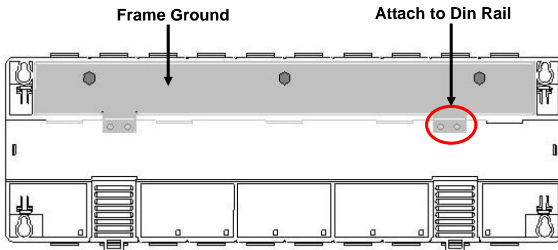
Fig. 29 : Frame Ground
