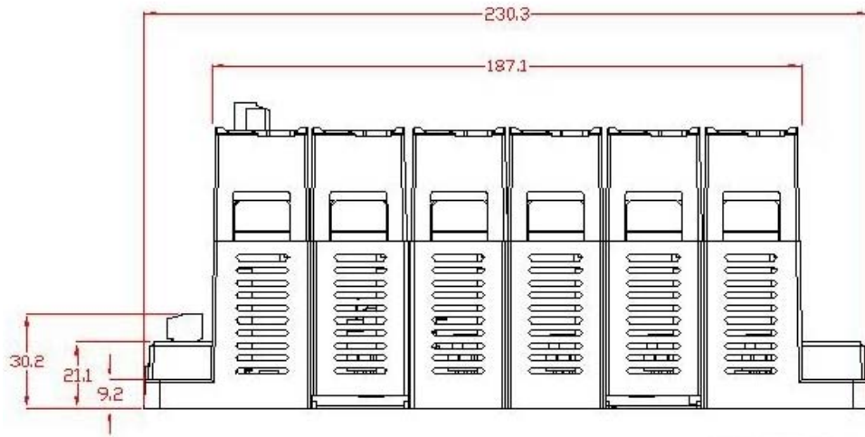
Bottom View
